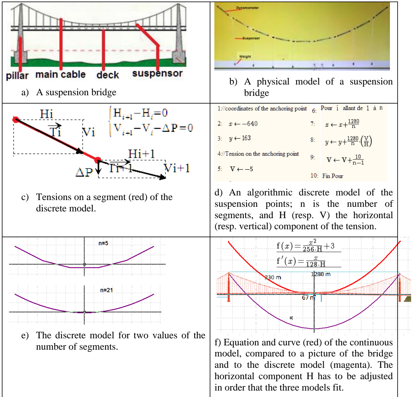
Figure 1: models of a suspension bridge
